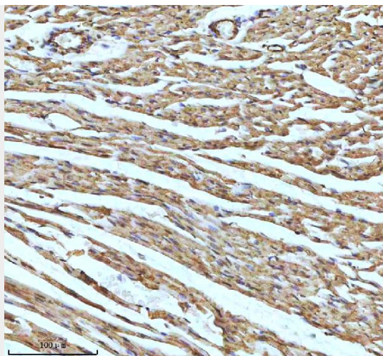
Figure 5. IHC analysis of UQCRFS1 using anti-UQCRFS1 antibody (M08781-1).
